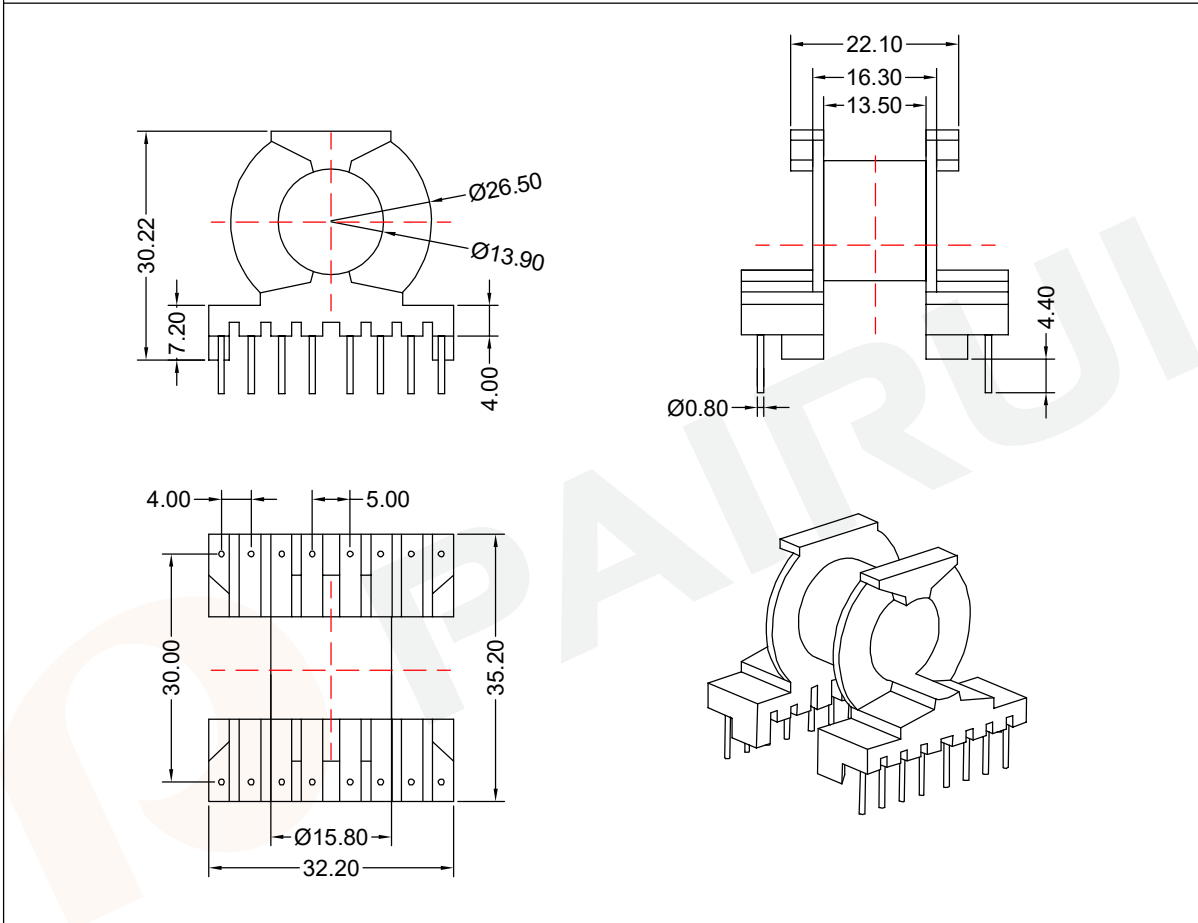
Winding data and area product for 16-pins PQ32/25 coil former
