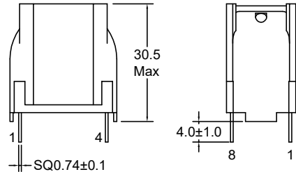
Orthographic view
