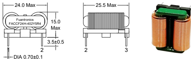
Orthographic view
