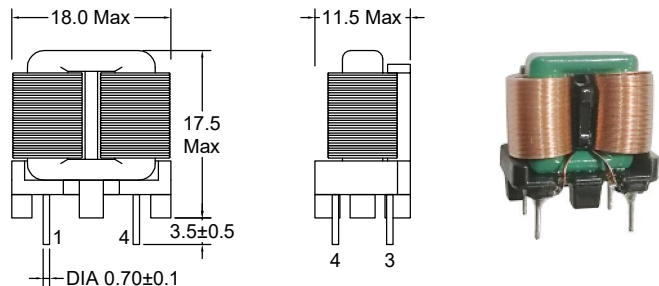
Orthographic view
